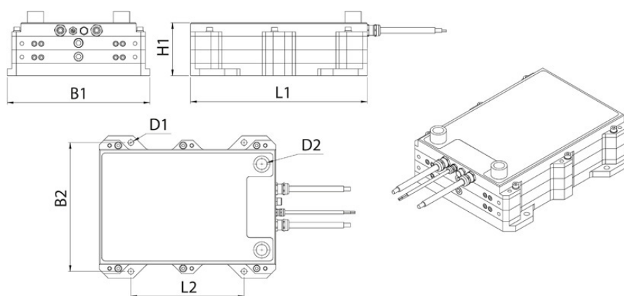
Dimension drawing
