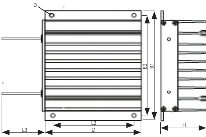
Design IP 20
