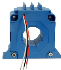
WKO-2C-A-K-L Model with front cover, litz wire and mounting feet lateral
