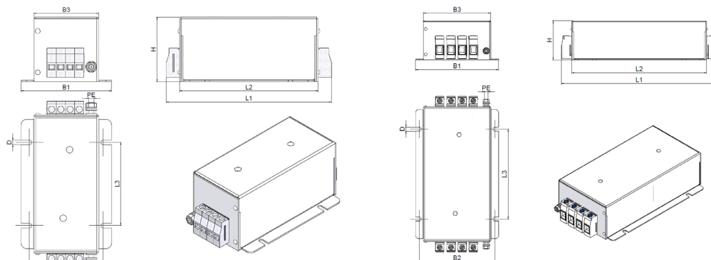
Housing B
