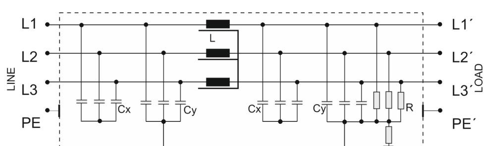
Circuit example
