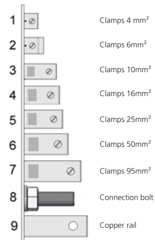
PE-Connections
