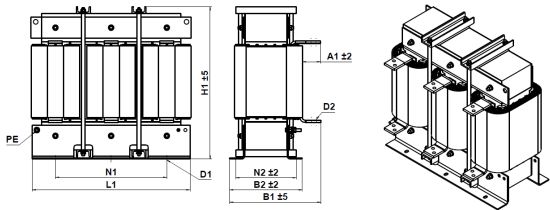
Design 6
