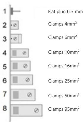
PE-Connections
