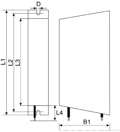
Standing view
