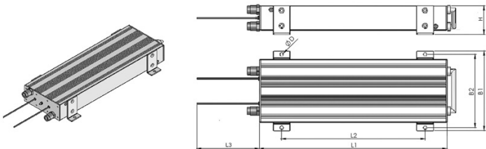
Dimension drawing, Design 1
