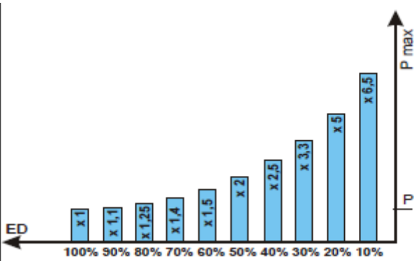
Load diagram
