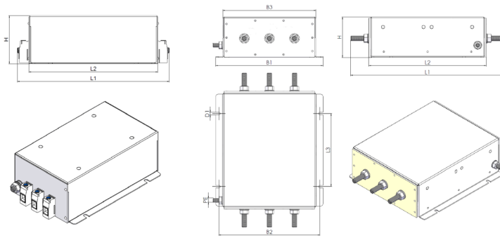
Housing C
