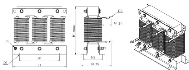
Design 3
