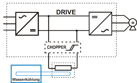
Circuit example
