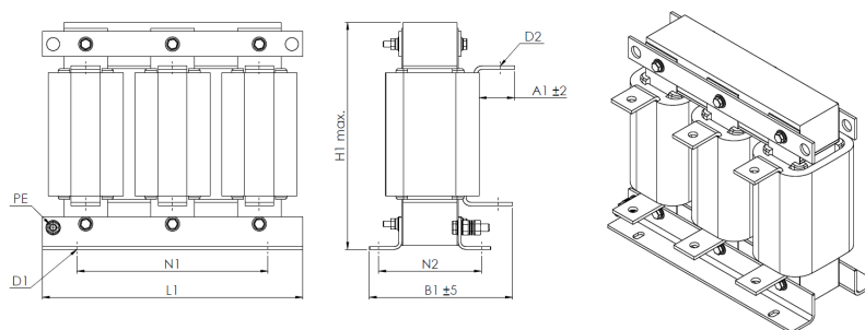
Design 3
