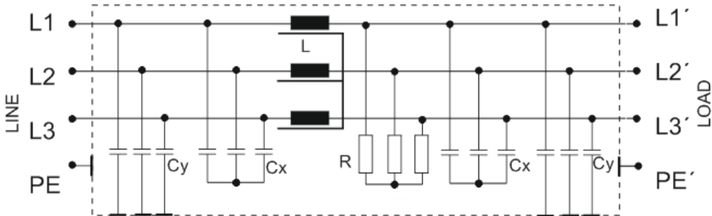
Circuit example
