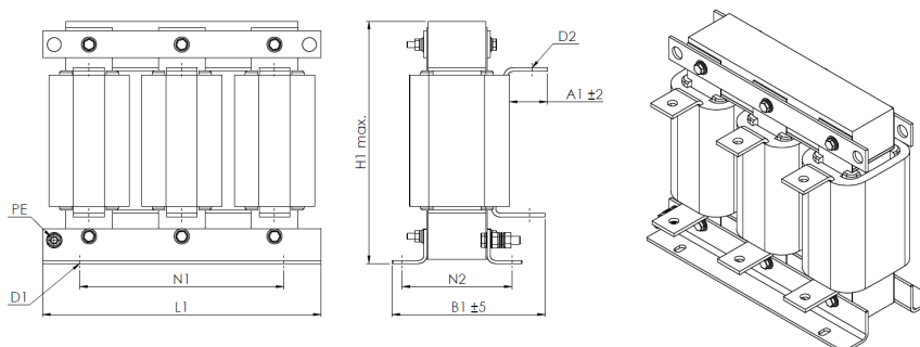
Design 3
