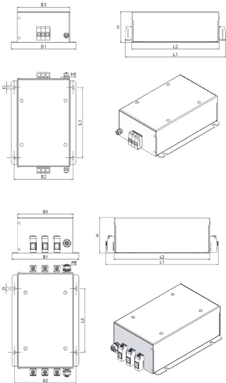
Housing B
