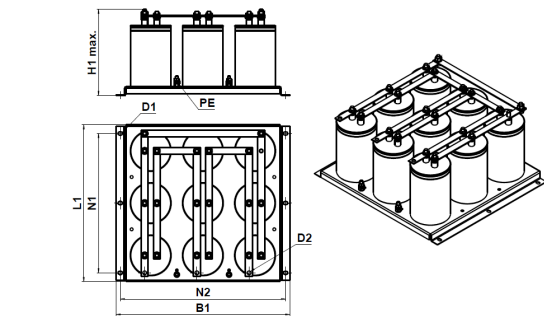
Design 7
