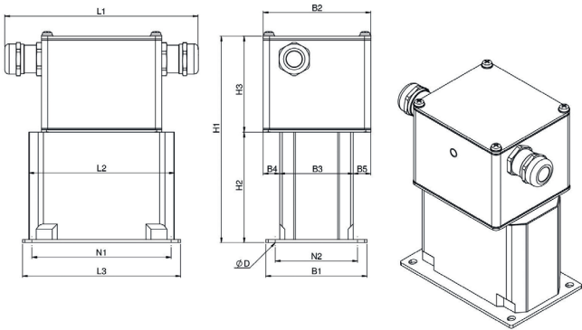
Design 1
